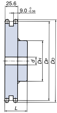
(Welded specifications) 2B type
