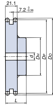
(Machined specifications) (Welded specifications) 2B type
