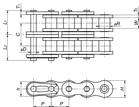
Double strand
