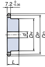
(Machined specifications) 1B Type
