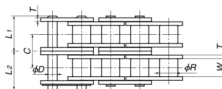
Double strand
