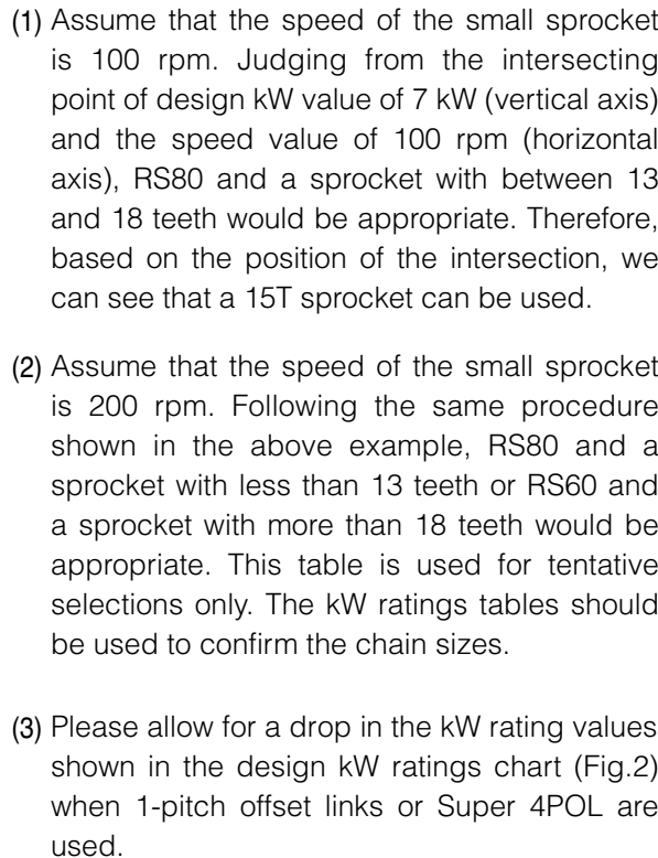
■ How to use this table (Fig. 2) 1. Example: Single-strand chain, design kW=7kW
