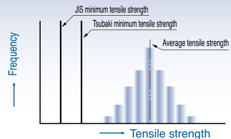
Fig. 1 Relationship between three tensile strengths
