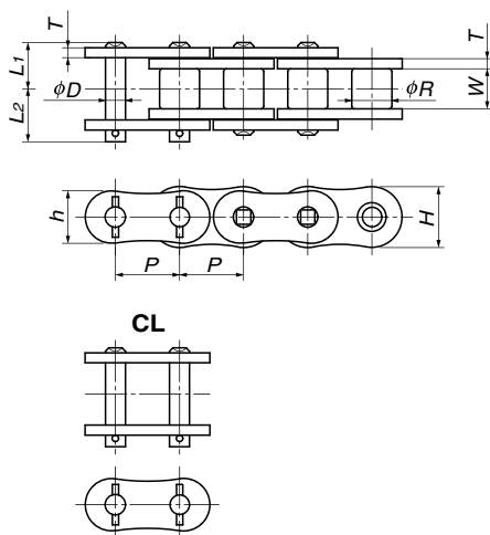
Single strand
