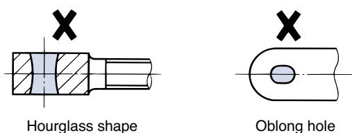
Fig. 30 Wear on the end fitting hole
