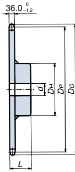
Welded construction 1B type
