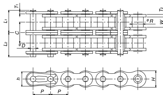
Double strand
