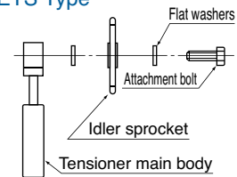
Fig. 1 Chain tensioner assembly
