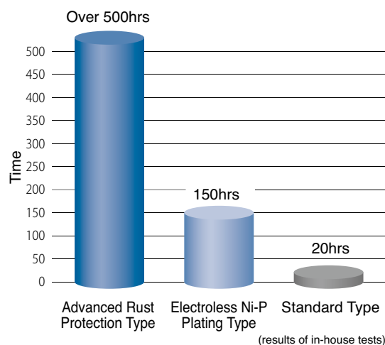
Comparison of Appearance of Red Rust in SST Tests
