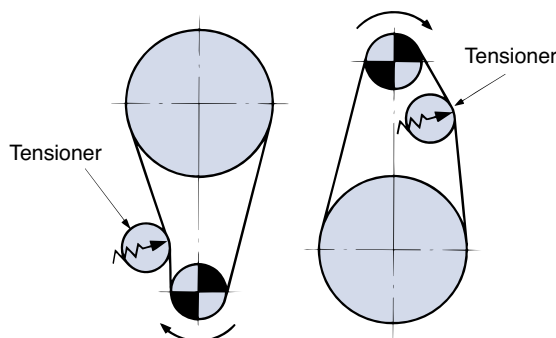
Fig. 22 Vertical transmission
