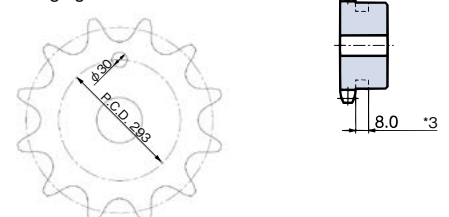
Hanging hole dimensions
