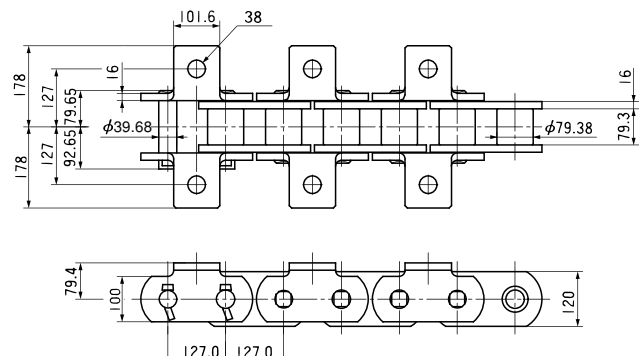
RS400-T-K1 Attachment Chain
