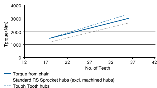
Comparison of Hub kW Ratings
