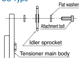
Fig. 1 Chain tensioner assembly
