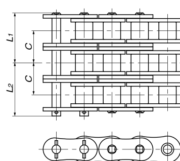
Triple strand
